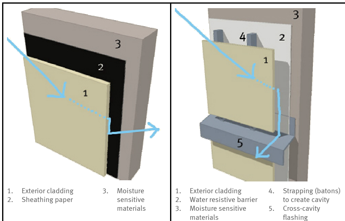
Figure 1: Face Seal Wall Assembly
