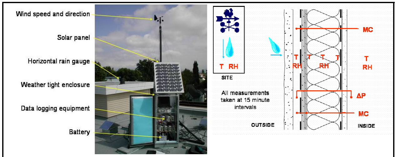
Figure 3: Monitoring Equipment and Sensor Locations
