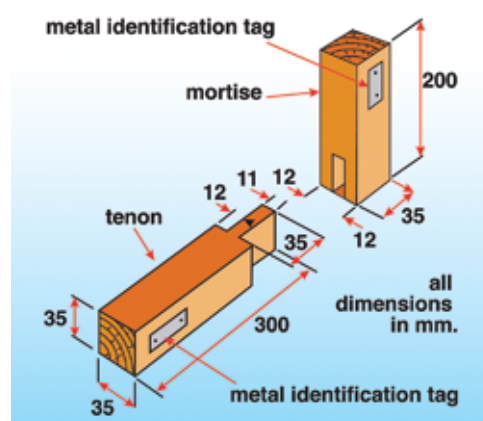
Figure 5. The L-joint specification.
