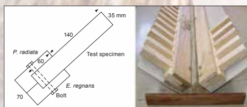
Figure 6. The embedded test in tilted orientation.
